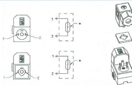
*Tilkoblingsbelegg Reed-bryter
