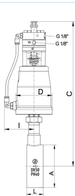
P/P-positionsregulator Type 8047
