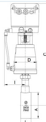
digital positionsregulator Type 8049
