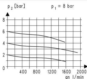
Flowdiagram
