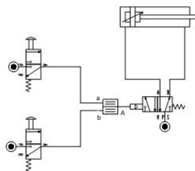
Connection diagram
