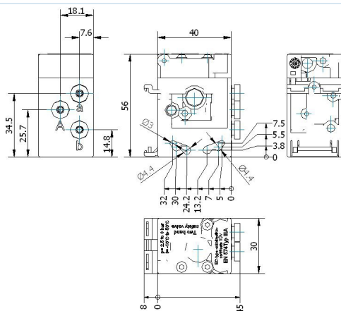
Dimensional drawing
