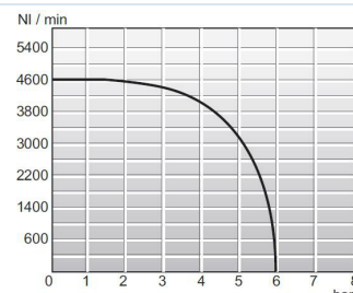
Dijagram protoka 1/2"
