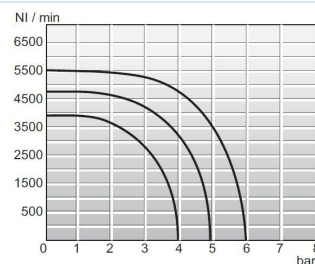
Flowdiagram 1/2"
