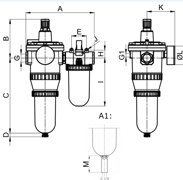
A1: automatic drain valve
