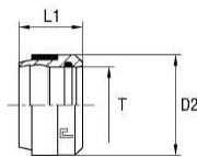
B4-Cutting ring
