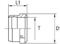
B3-Cutting ring
