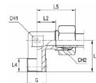
with B3 cutting ring
