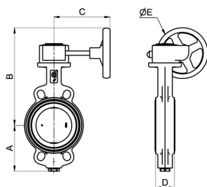
Sandwich mounting version
