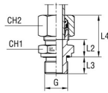
with B4 cutting ring
