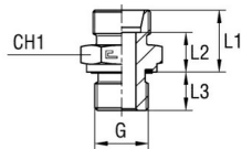
Main body
