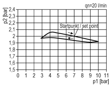
pressure characteristic
