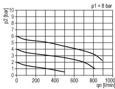
flow characteristic
