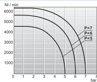
Flow diagram 1/2"
