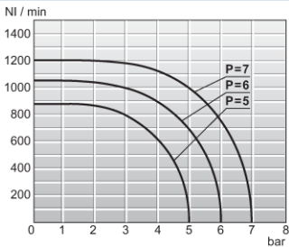
Flow diagram 1/8"
